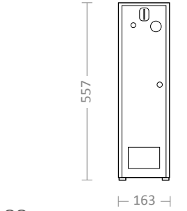
CC Coin Changer 18 kg
