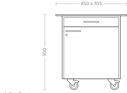
Mobile Cart Available: Water Self Supply / Flojet Pump / Water Filter 55 kg
