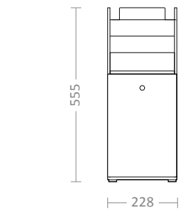
Ls Dispenser / 4 l Refrigerator 18 kg | 230 V | 0.08 kW
