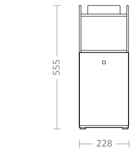
Lv Cup Warmer / 4 l Refrigerator 21 kg | 230 V | 0.16 kW
